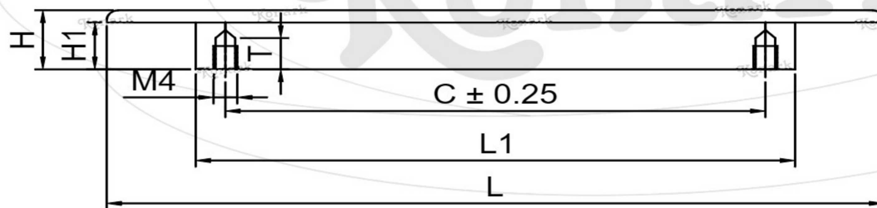
FRONT View
