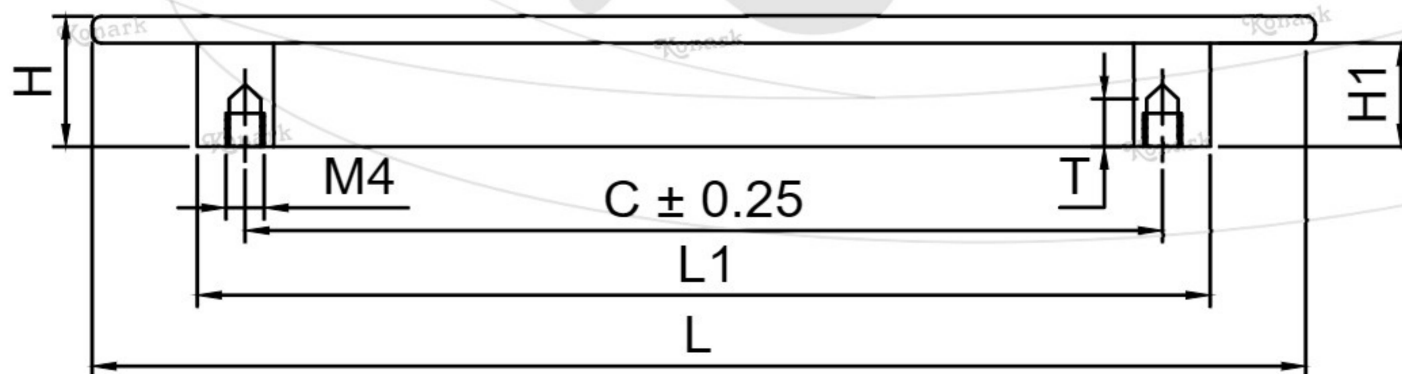
FRONT View
