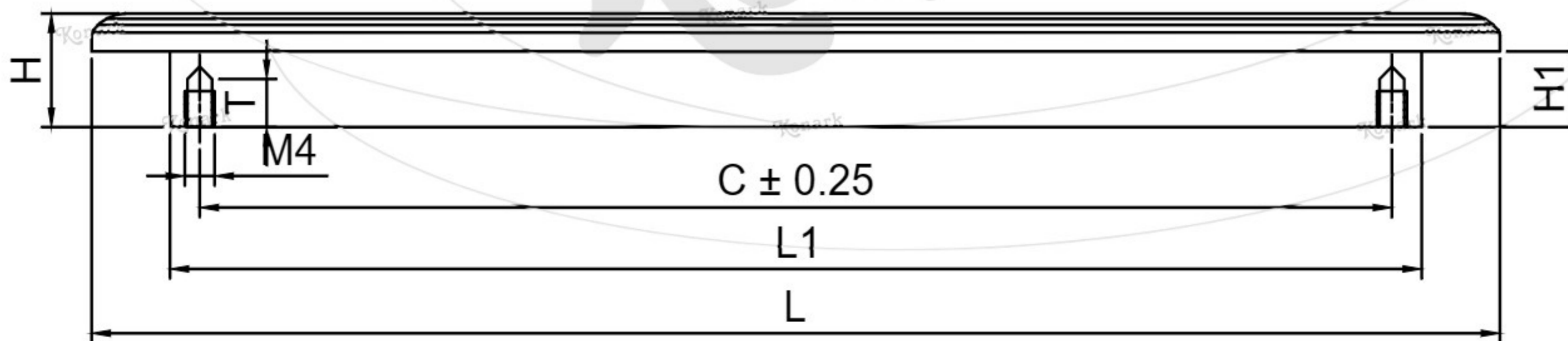
FRONT View
